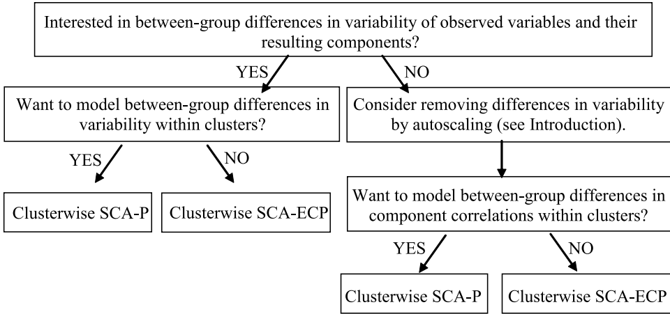
Figure 1. Decision tree for making the choice between applying clusterwise SCA-ECP and clusterwise SCA-P for a specific data analysis problem.
