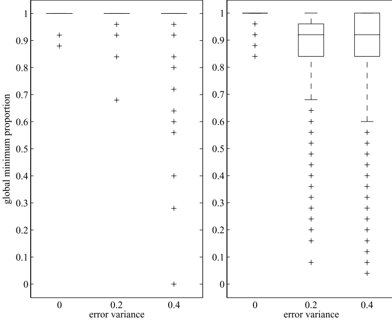
Figure 2. The proportion of random runs with a loss function value equal to that of the proxy of the global minimum ('global minimum proportion') as a function of the amount of error e when the number of clusters C is two (left panel) and when C is four (right panel).
