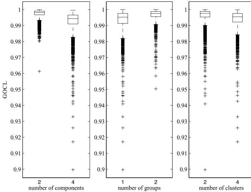
Figure 3. Box plots of the goodness-of-cluster-loading-recovery statistic (GOCL) as a function of the number of components (left), the number of groups (middle), and the number of clusters (right).
